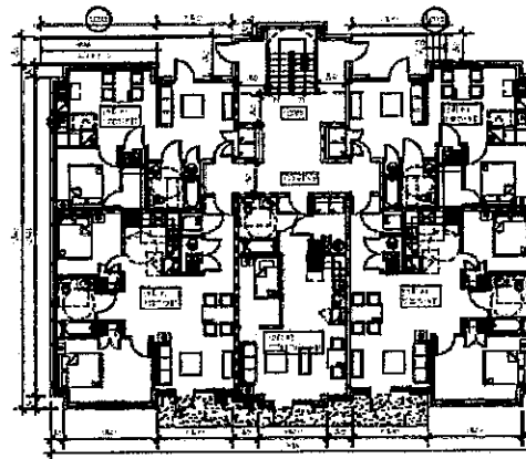
2 PROPOSED FIRST FLOOR PLAN SCALE 1/8" = 1'-0"
